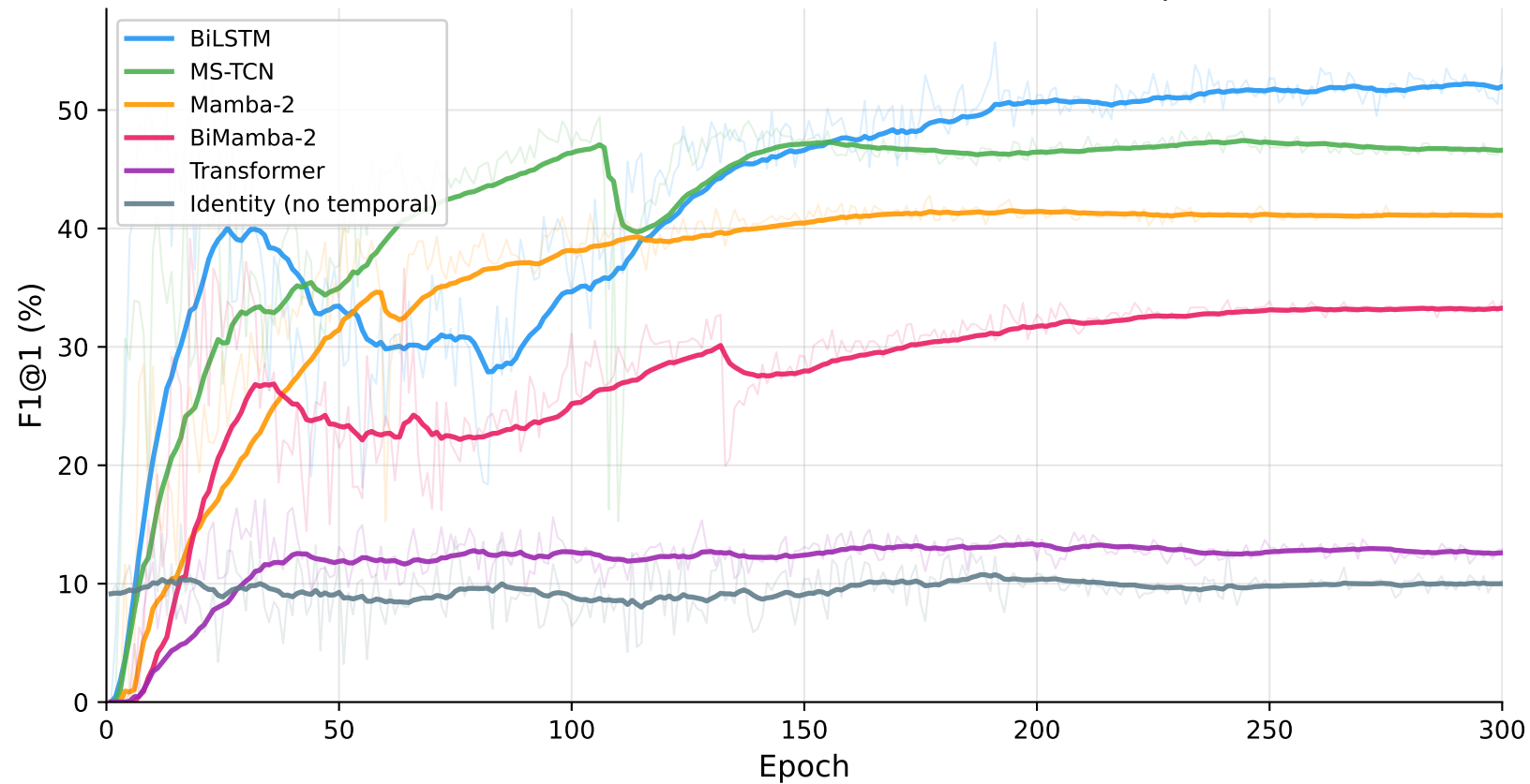
Hit Detection F1@1 (EMA smoothed, \alpha=0.92 ) — All Temporal Heads
