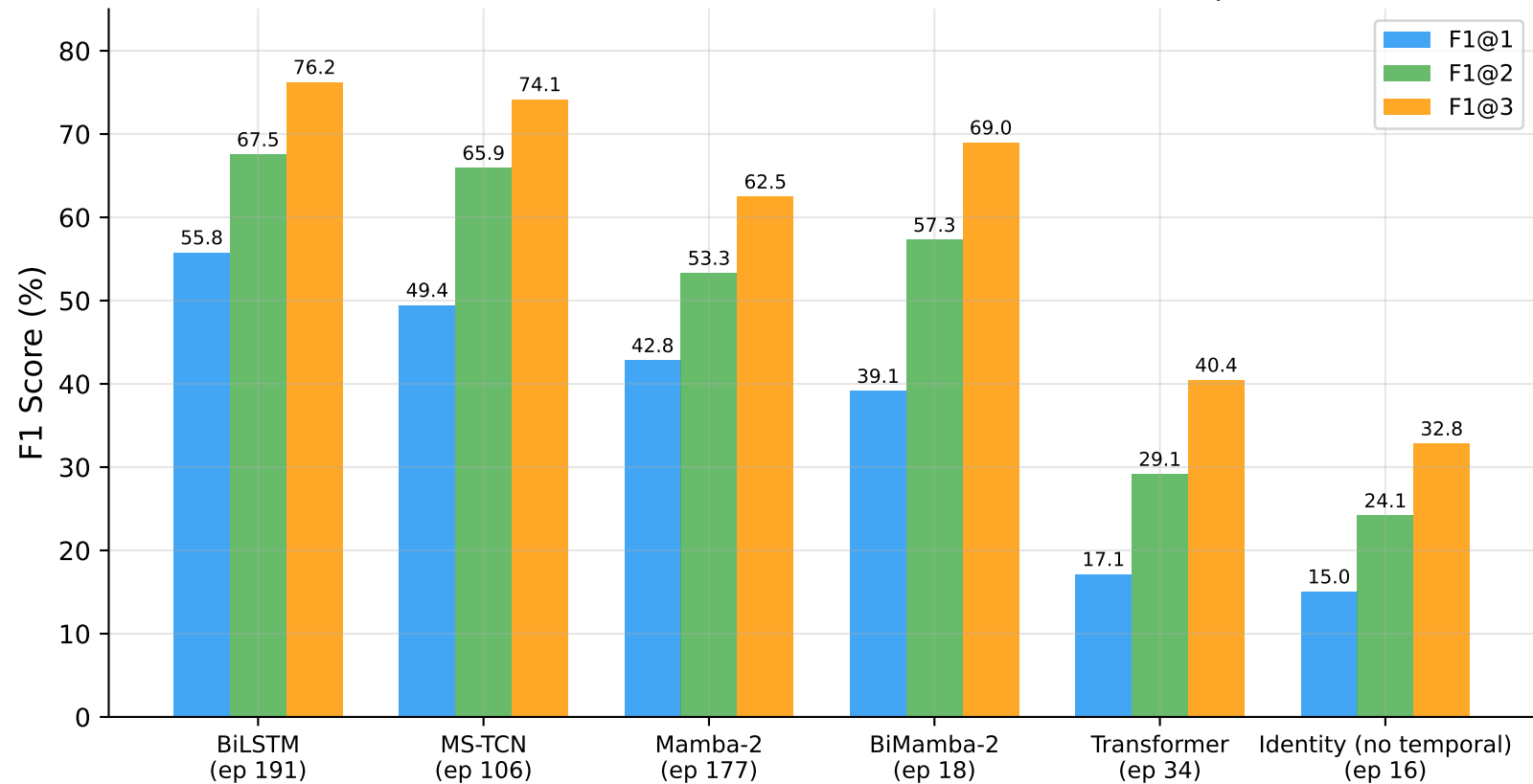
Best F1 Scores at \pm 1/\pm 2/\pm 3 Frames (at Best F1@1 Epoch)
