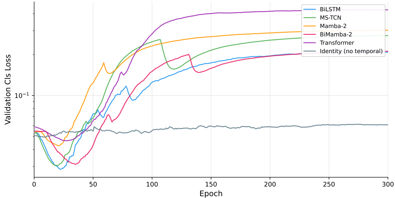
Validation Classification Loss (EMA smoothed) — All Heads
