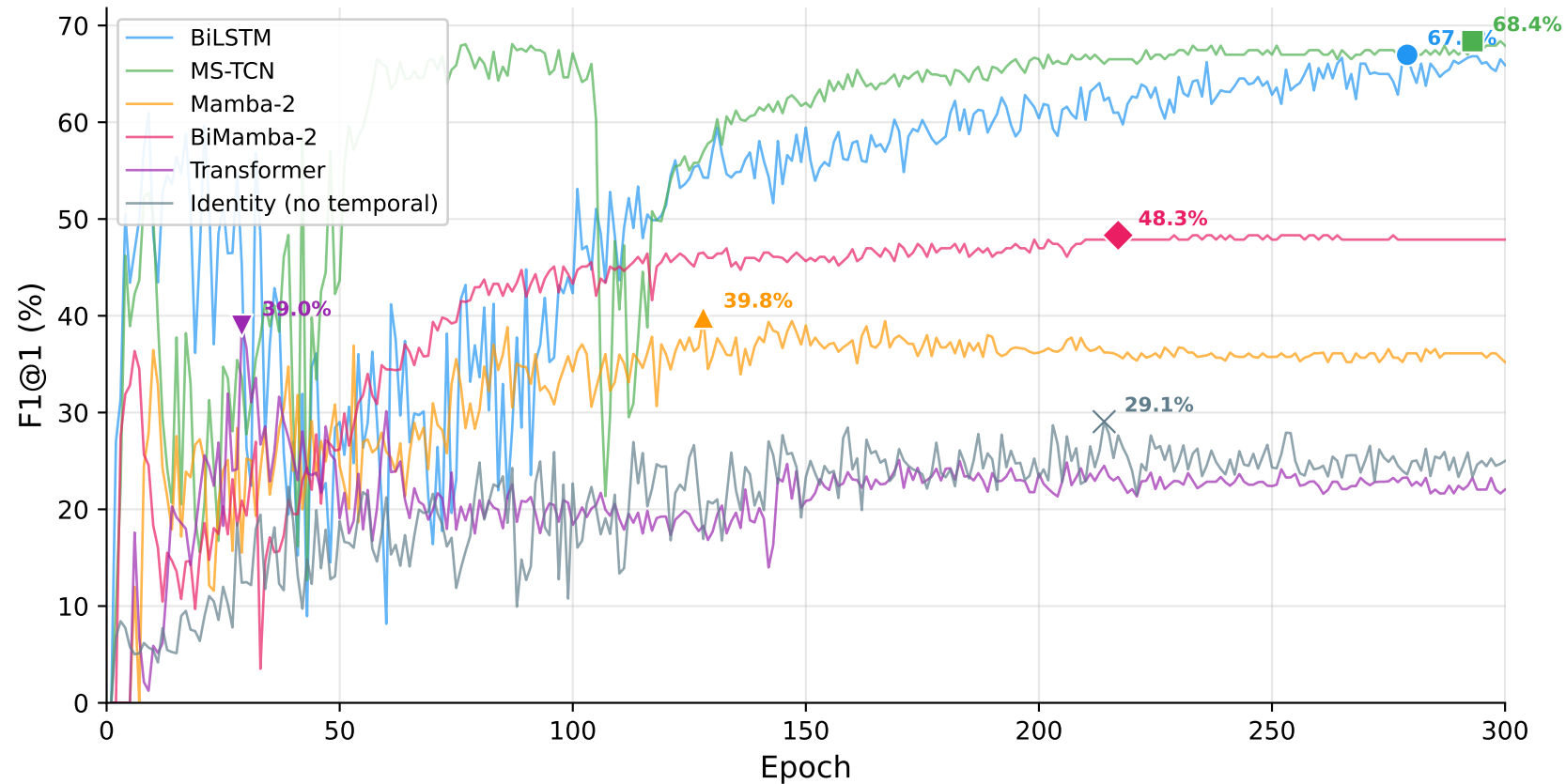
Hit Detection F1@1 ( \pm 1 frame) — CE-518 Features
