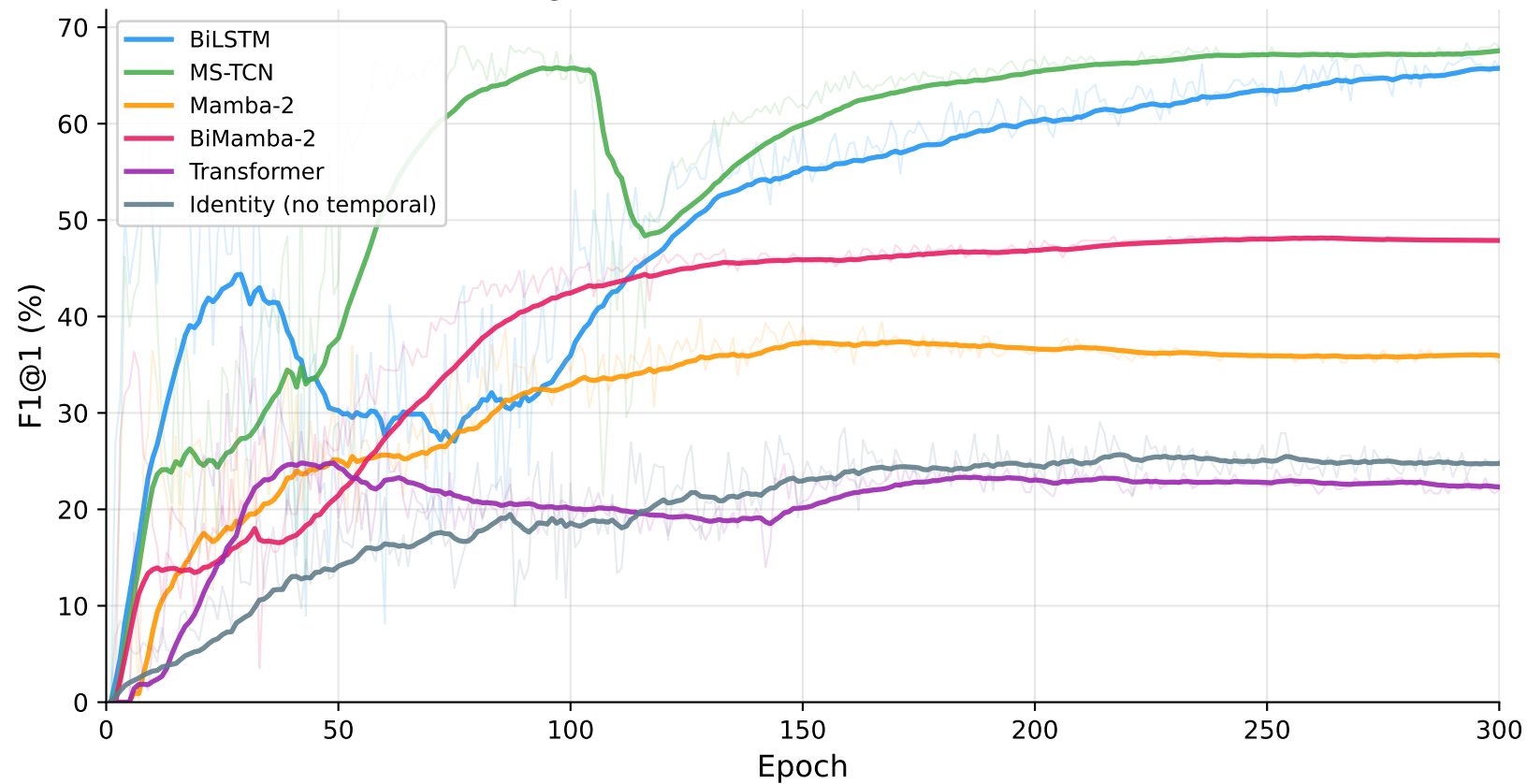
Hit Detection F1@1 (EMA smoothed, \alpha=0.92 ) — CE-518 Features
