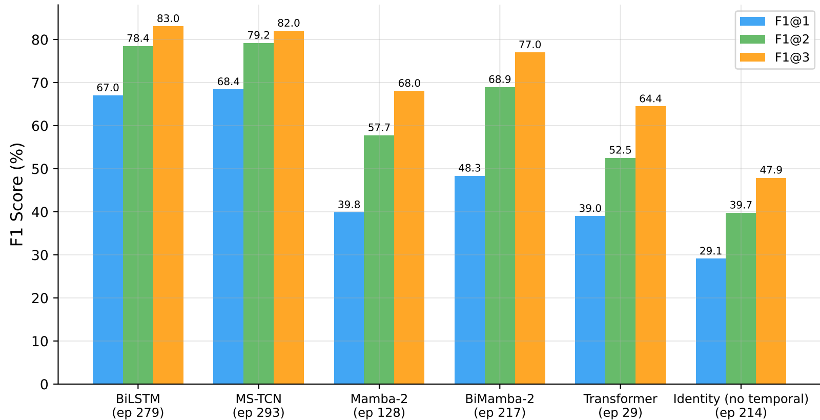
Best F1 Scores at \pm 1/\pm 2/\pm 3 Frames — CE-518
