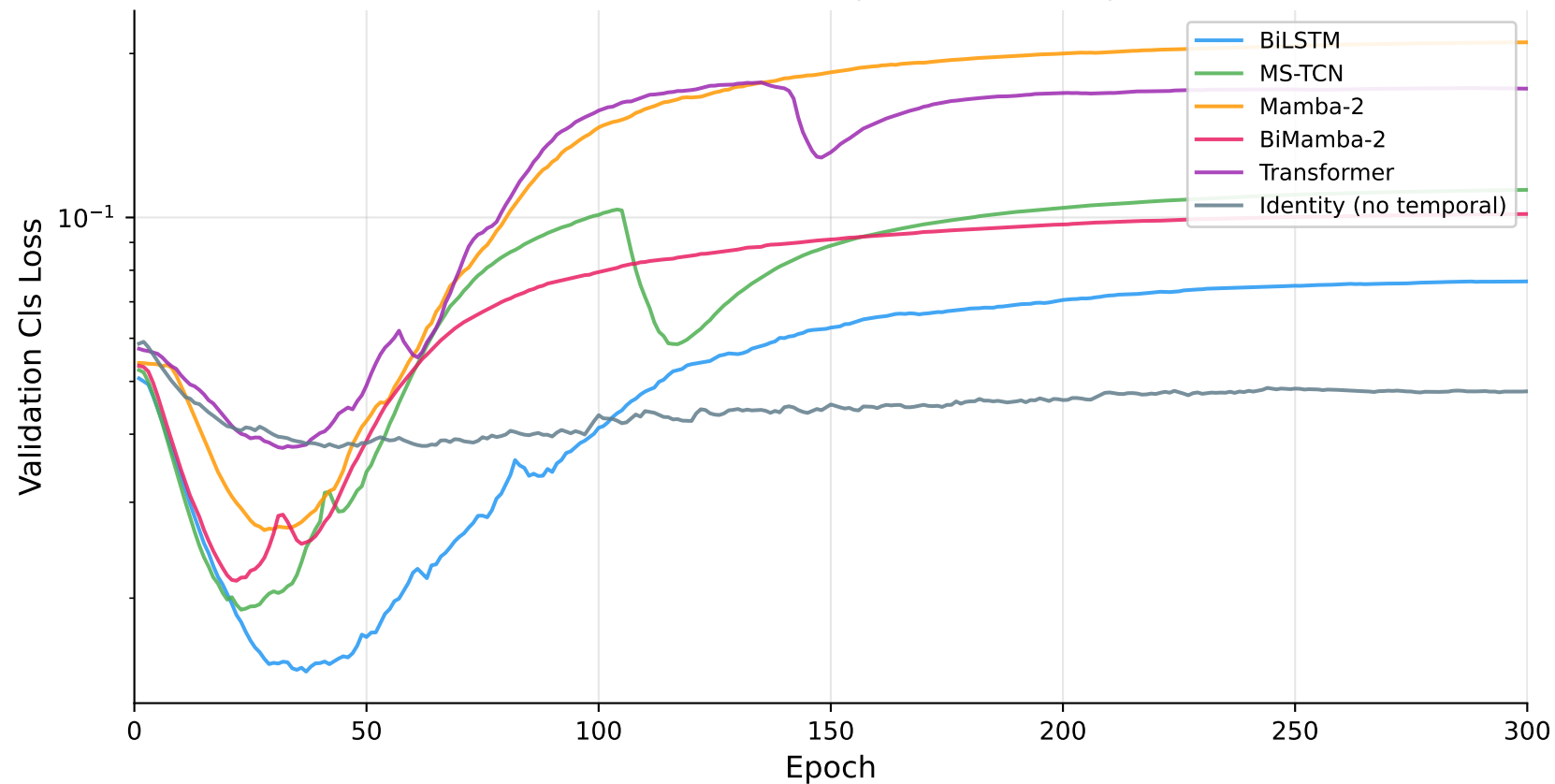
Validation Classification Loss (EMA smoothed) — CE-518
