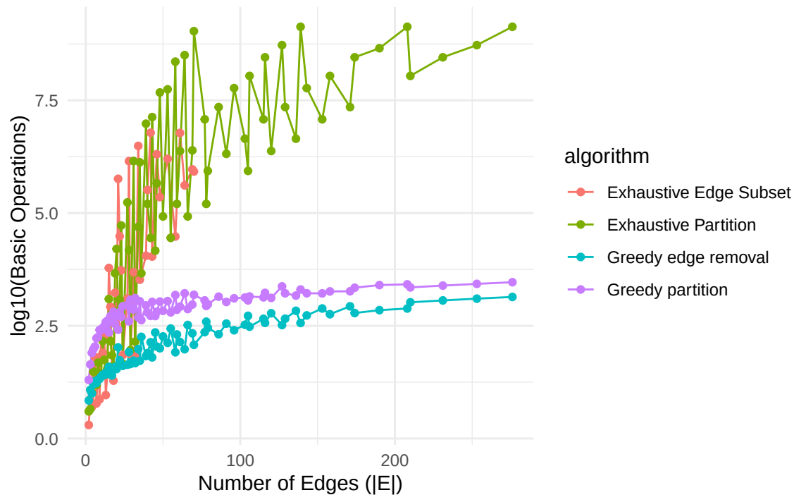
Log Basic Operations vs Number of Edges
