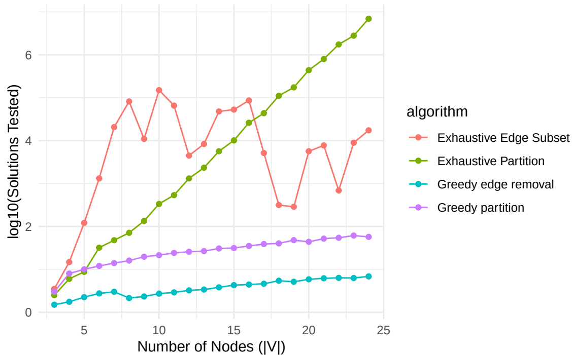
Log Solutions Tested vs Number of Nodes
