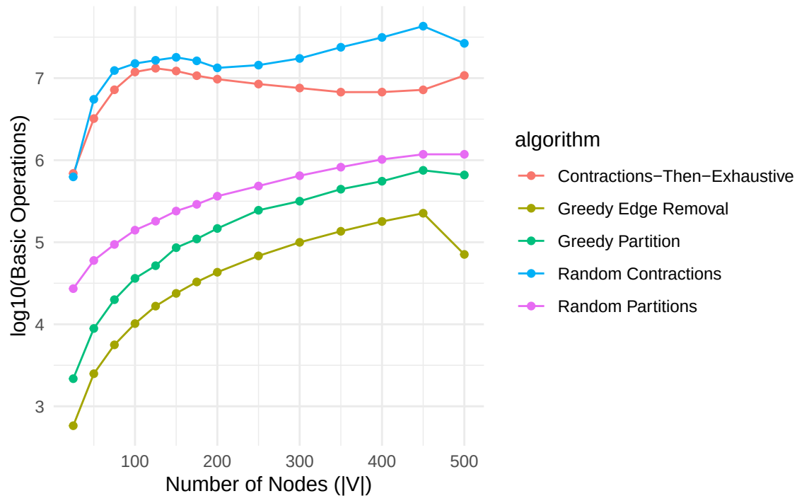
Log Basic Operations vs Number of Nodes
