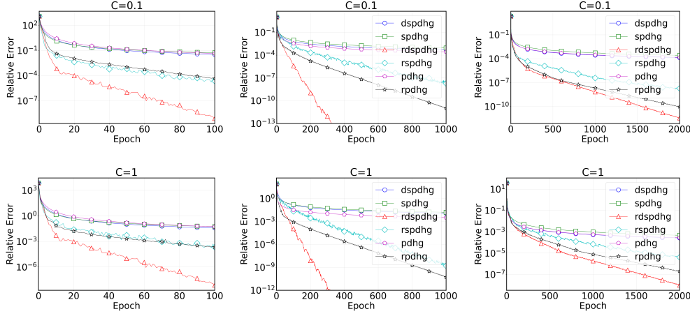
Fig. 1: Relative error for soft-margin SVM. First column: colon-cancer ( n = 62, m = 2000 ) with p = 0.3, q = 0.15 ; second column: mushrooms ( n = m = 100 ) with p = q = 0.1 ; third column: w1a ( n = 2477, m = 300 ) with p = 0.2, q = 0.4 .
