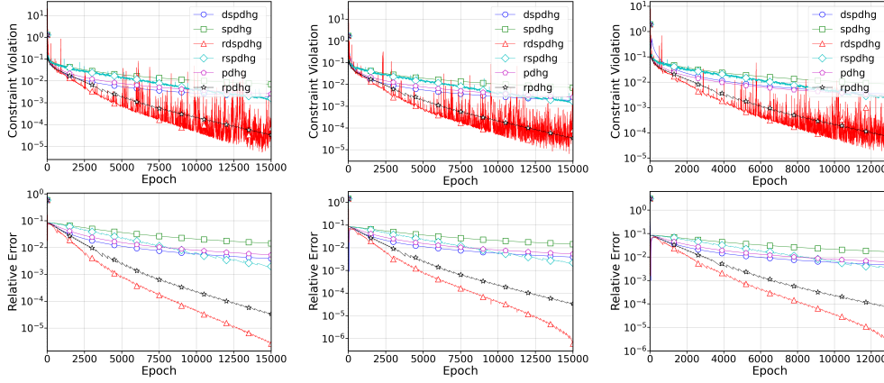
Fig. 2: Constraint violation and relative error for MPC problems with n_x = n_u = 20 and p = 0.1, q = 0.5 . First column: T = 20 ; second column: T = 50 ; third column: T = 100 .
