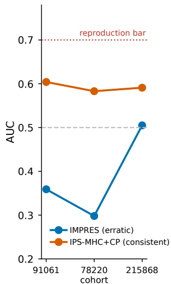
(c) 3 — Direction consistency
