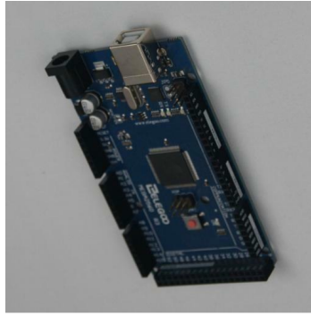
(b) Mega 2560 variant 2
