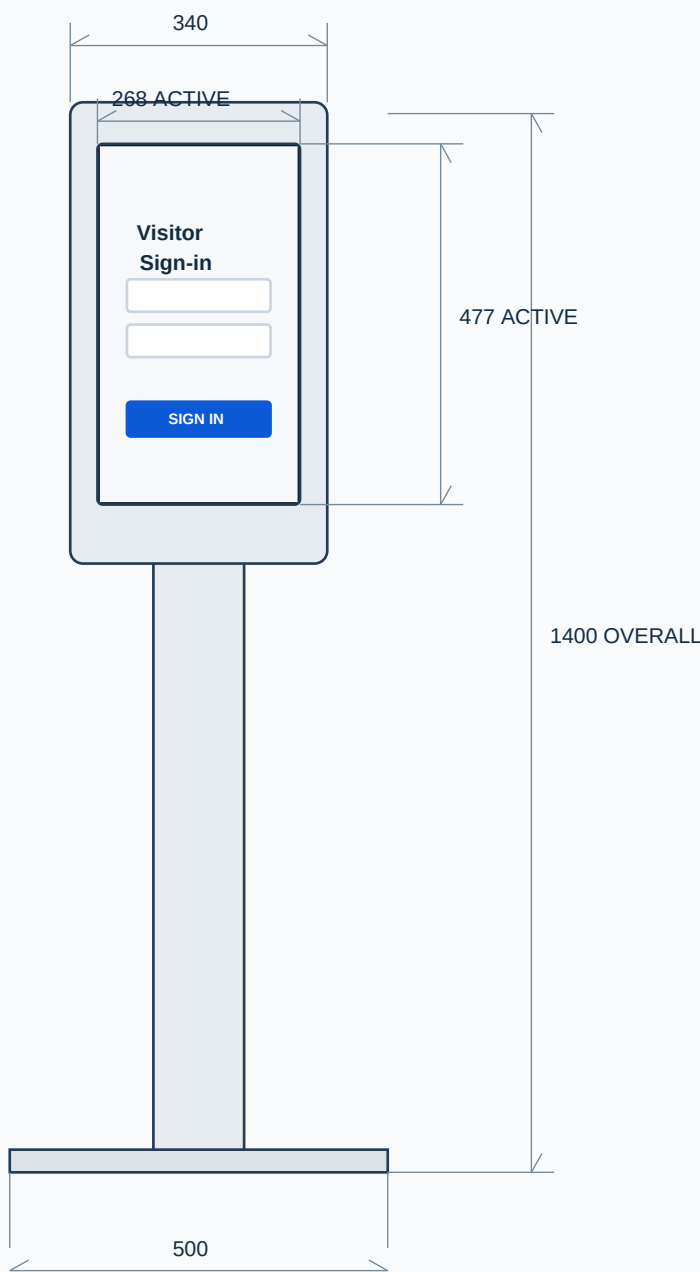
FRONT ELEVATION
