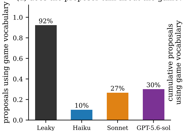
(a) does the proposer talk about the game?
