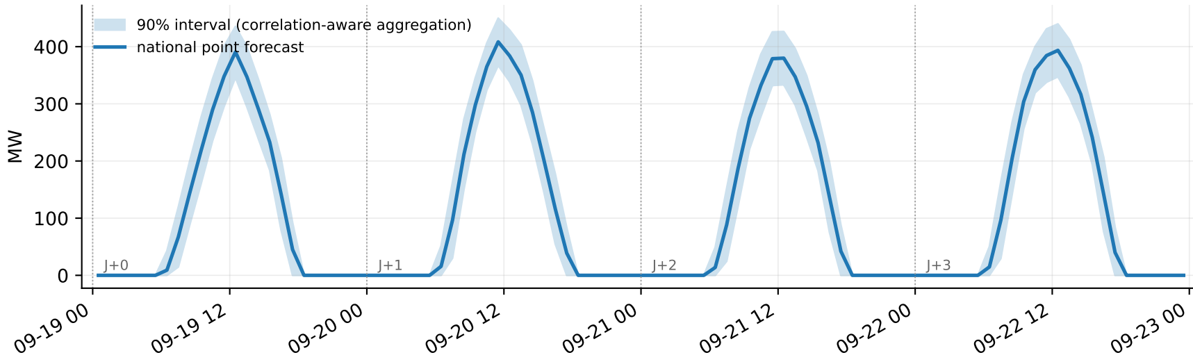
National rooftop PV forecast, J+0 to J+3, with aggregated uncertainty
