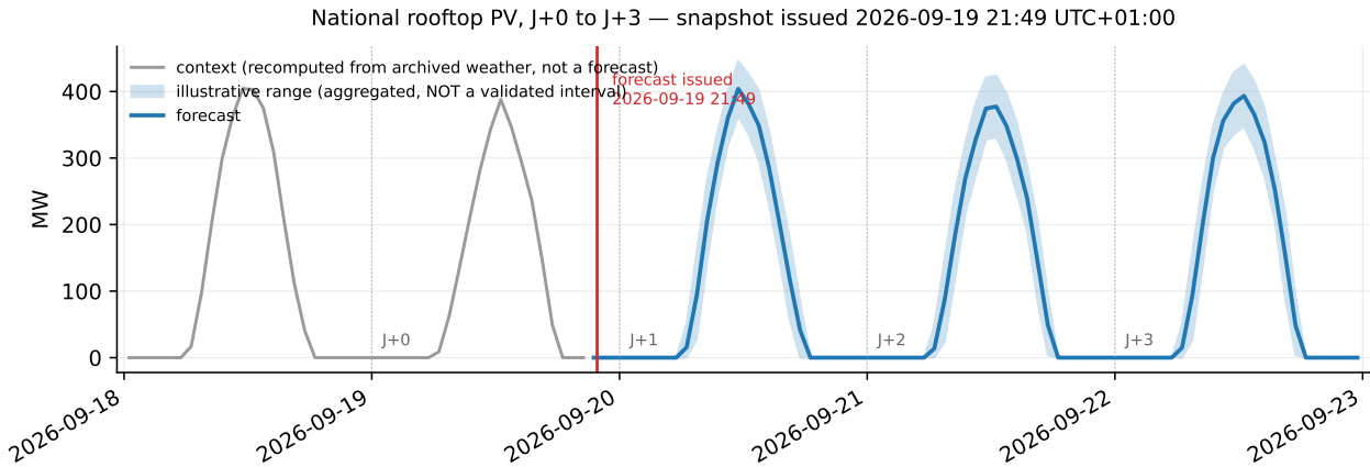
Figure 4: The product, from the snapshot issued 2026-09-19 21:49 that every number in this report is drawn from. The red line is the issue time , and J+0 is counted from it. Hours to its left are context : values recomputed from archived weather for elapsed hours, drawn in grey and not forecasts of those hours — a freshly generated estimate for an hour that has already passed is not an operational forecast of it. The shaded band on the forecast side is the illustrative range of §3.3, not a validated 90% interval. The snapshot holds 69 context hours and 146 forecast hours.
