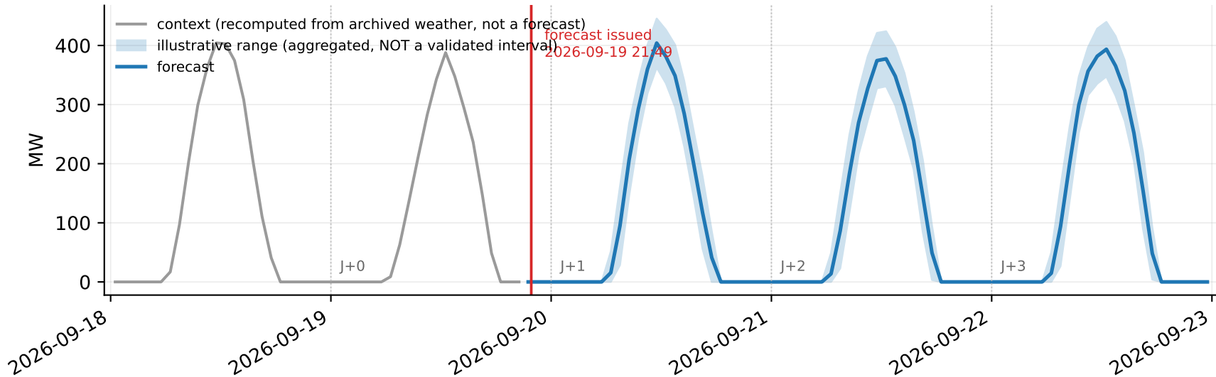
National rooftop PV, J+0 to J+3 — snapshot issued 2026-09-19 21:49 UTC+01:00
