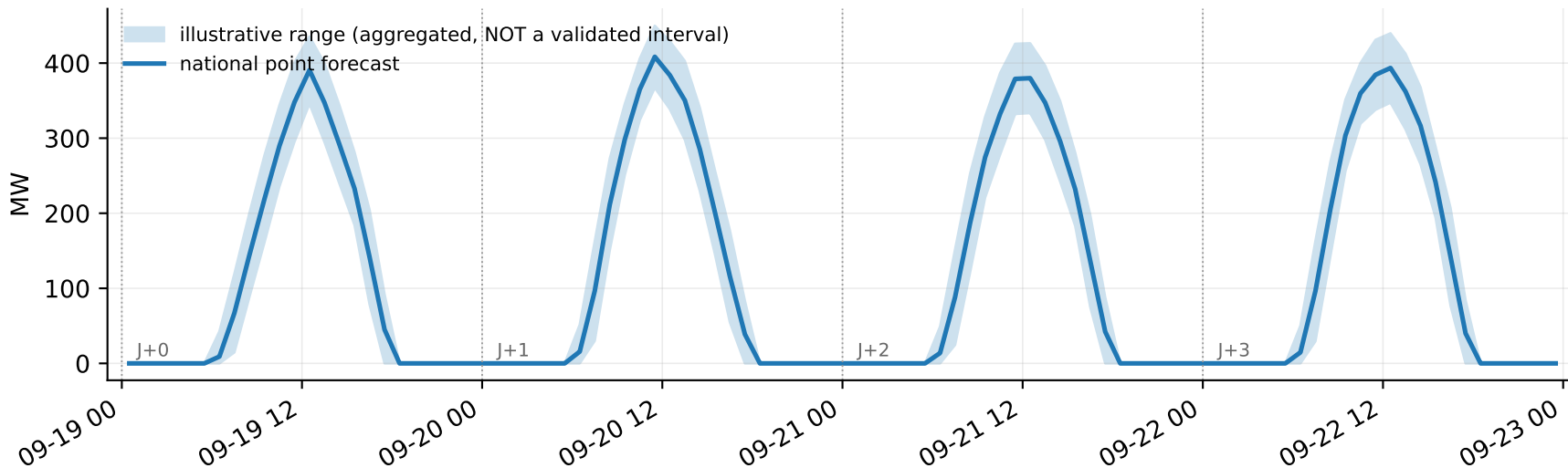
National rooftop PV forecast, J+0 to J+3 (forecast issued 2026-09-19 21:22 UTC+01:00)
