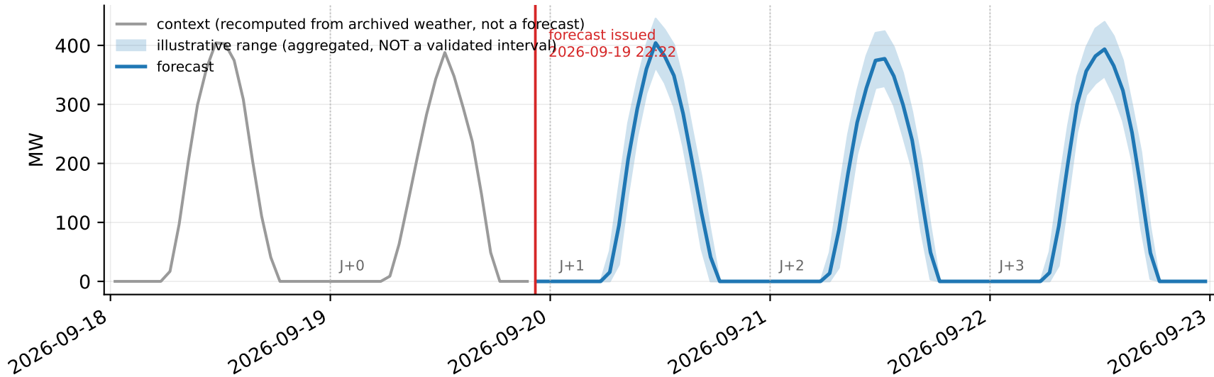
National rooftop PV, J+0 to J+3 — snapshot issued 2026-09-19 22:22 UTC+01:00
