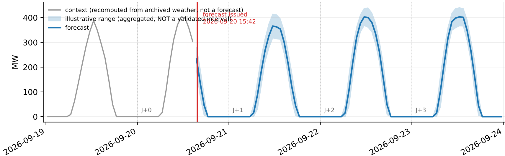
National rooftop PV, J+0 to J+3 — snapshot issued 2026-09-20 15:42 UTC+01:00
