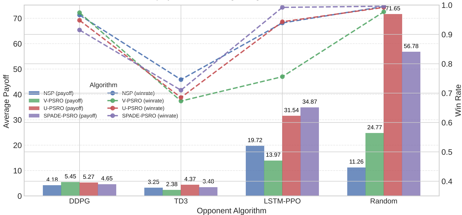
Crossplay Performance against general rl baselines
