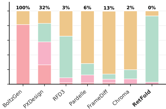
(b) Full-chain retrieval (qTM)
