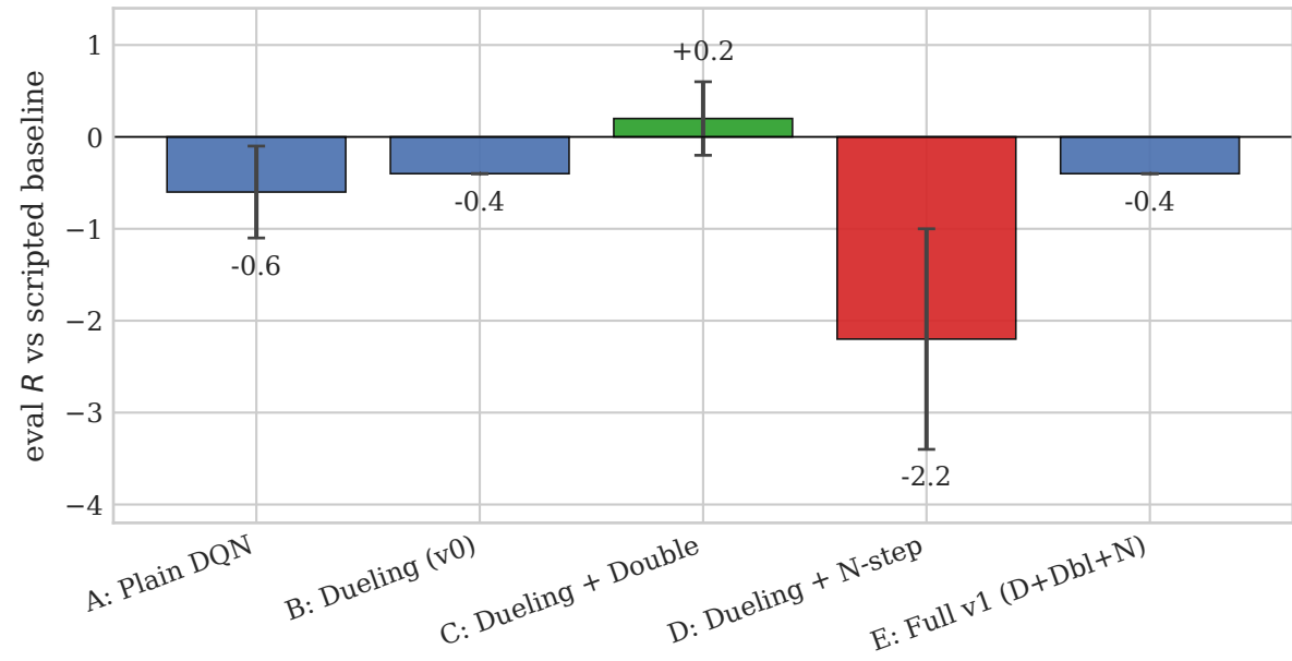
Component ablation: Dueling x Double x N-step (5M steps)
