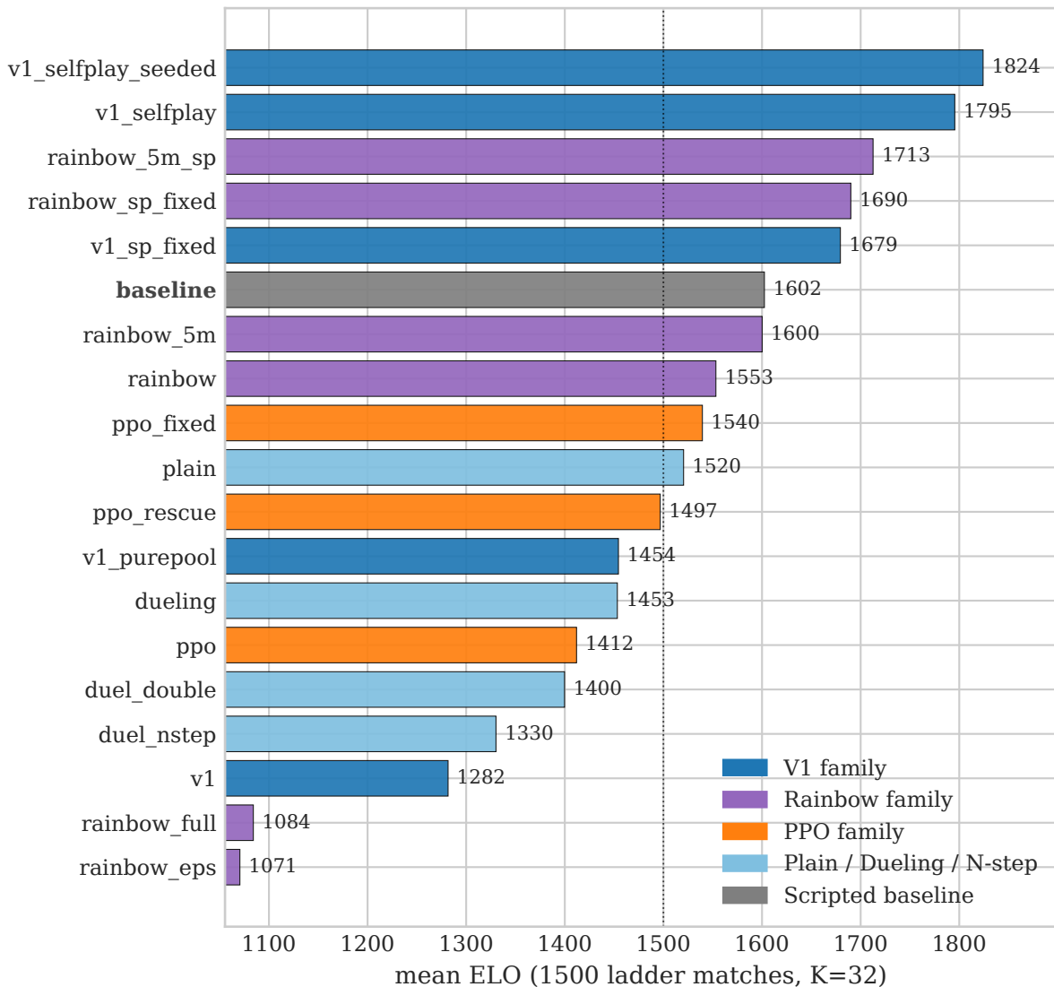
Per-variant aggregate ELO
