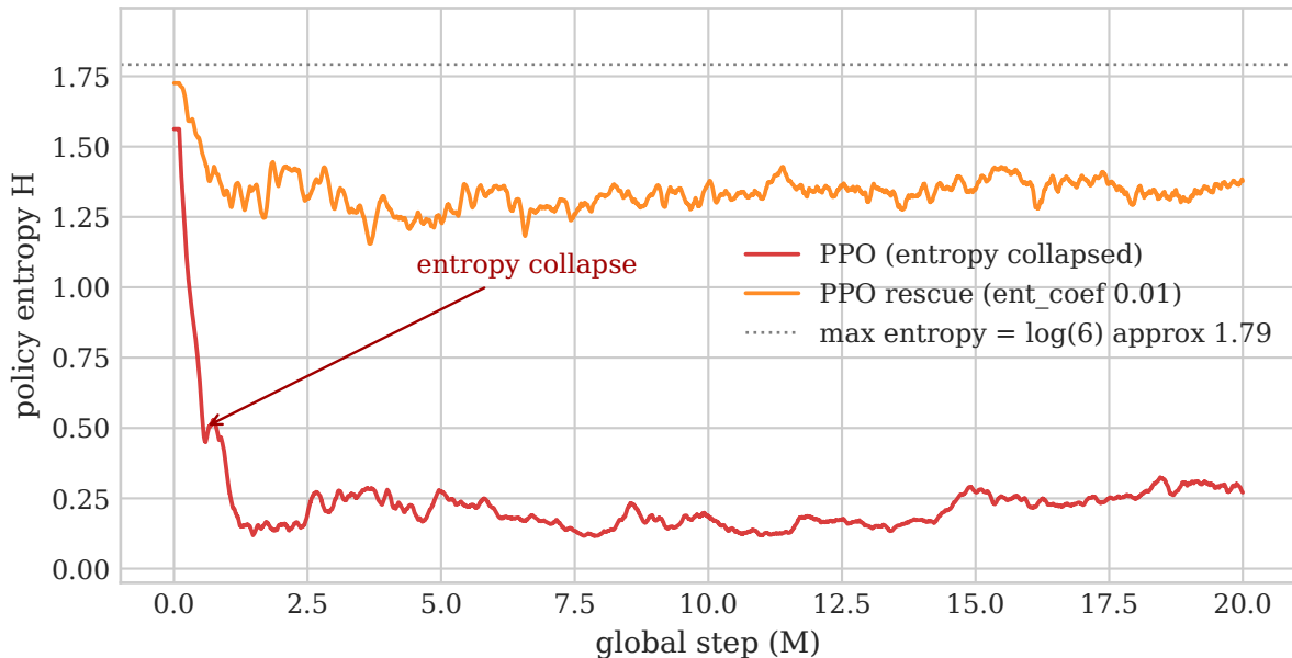
PPO policy entropy: collapse vs rescue
