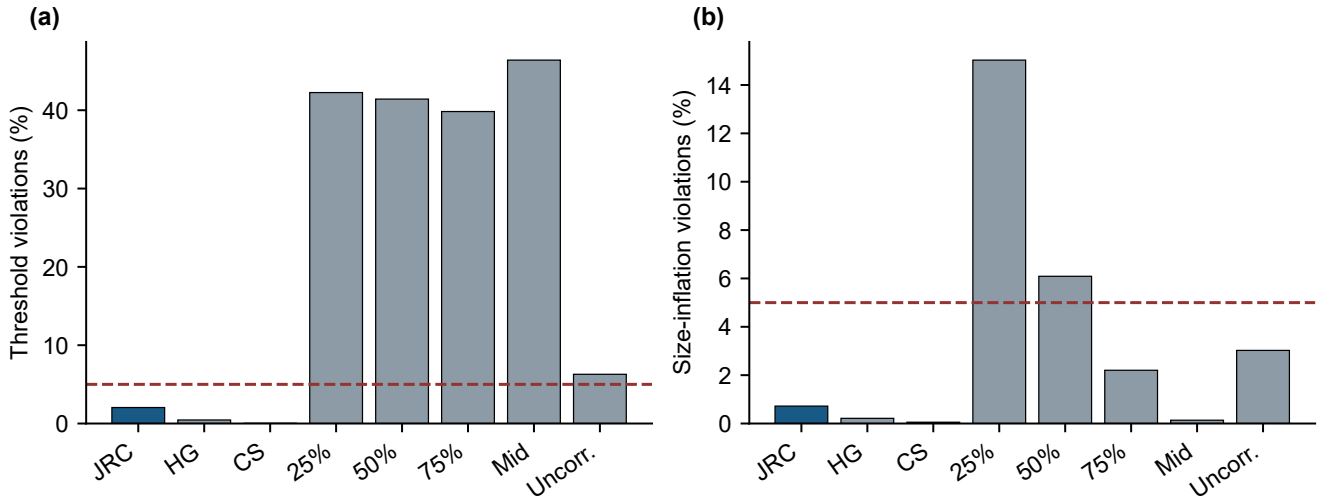
Fig. 3 USC-HAD LAC failure diagnostics: (a) output threshold below the full-reference threshold; (b) monitoring-batch inflation above 0.5 labels. The horizontal line marks 5%. Fixed fractions, midpoint output (Mid) and uncorrected repeated looks (Uncorr.) do not have the JRC contract
