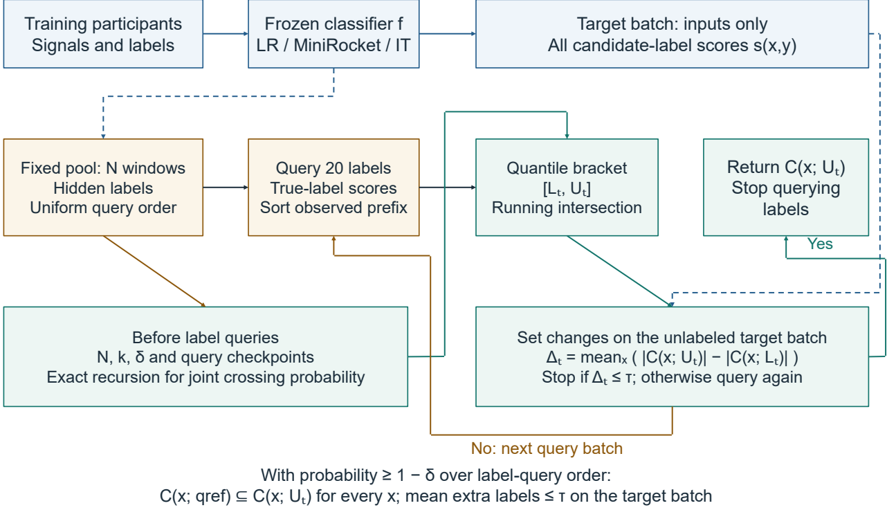
Fig. 1 Overall architecture of JRC. A frozen classifier supplies the class-score matrices. Offline rank boundaries depend on the pool size, reference rank, confidence error and declared checkpoints. The query loop returns a threshold with reference-set containment and batch-specific inflation control
