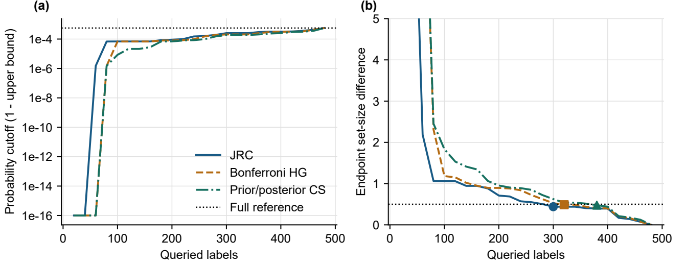
Fig. 6 First declared USC-HAD MR query run, LAC, 480 reference windows: (a) upper quantile endpoints represented as the corresponding probability cutoff 1 - U_t on a logarithmic axis; (b) endpoint set-size difference with stopping locations marked. The reference quantile is approximately 0.999436. Zero cutoffs and infinite upper bounds are displayed at 10^{-16} in (a); this is only a display convention. The horizontal line in (b) is the 0.5-label tolerance
