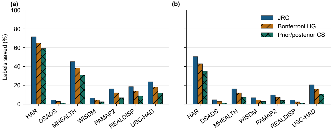
Fig. 2 Label savings at confidence error 0.05 and tolerance 0.5: (a) LAC; (b) APS. Solid, hatched and cross-hatched bars identify JRC, Bonferroni hypergeometric brackets and the primary uniform-prior confidence sequence. Values average the declared pool ceilings and participant summaries
