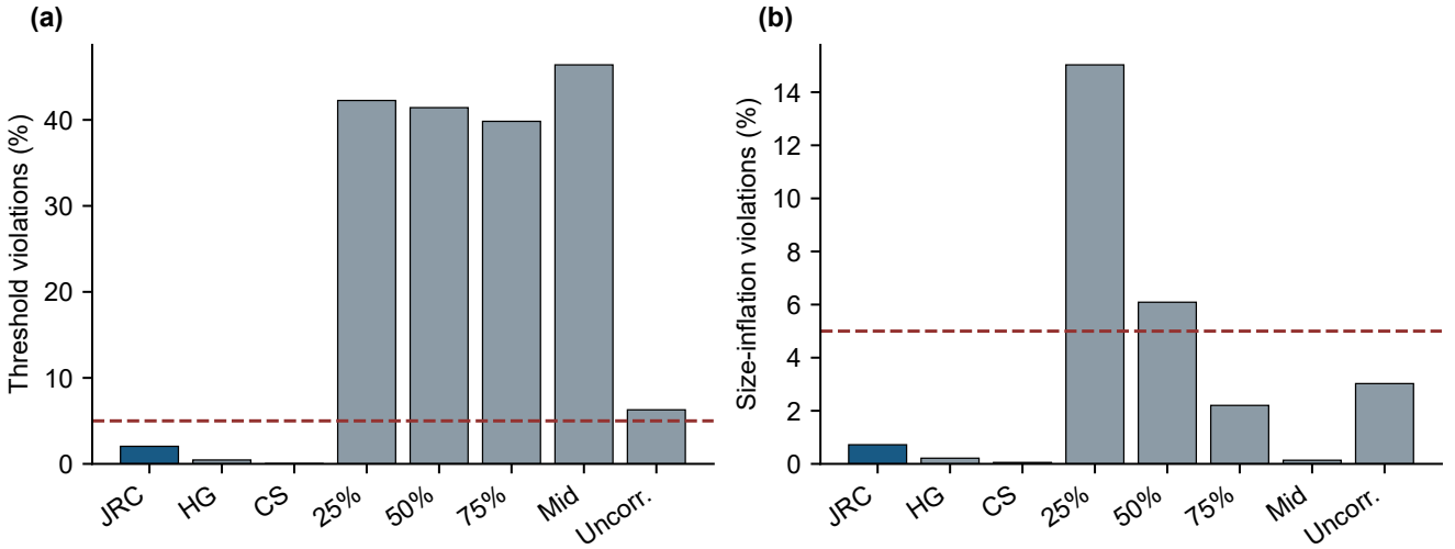
Fig. 3 USC-HAD LAC failure diagnostics: (a) output threshold below the full-reference threshold; (b) monitoring-batch inflation above 0.5 labels. The horizontal line marks 5%. Fixed fractions, midpoint output (Mid) and uncorrected repeated looks (Uncorr.) do not have the JRC contract
