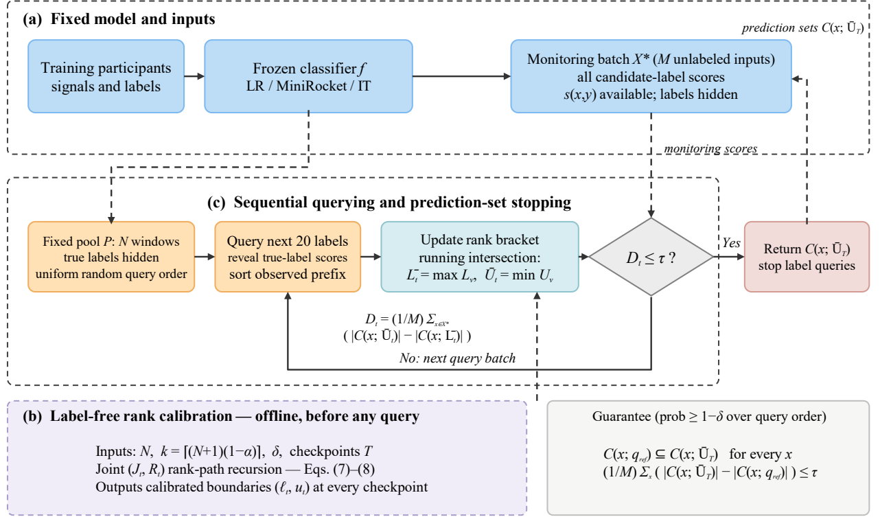
Fig. 1 JRC framework. (a) A frozen classifier provides candidate-label scores. (b) Joint rank calibration constructs checkpoint boundaries before querying. (c) Labels are queried uniformly without replacement to update the quantile bracket; querying stops when the endpoint sets meet the monitoring-batch size tolerance, and the upper-endpoint sets are returned
