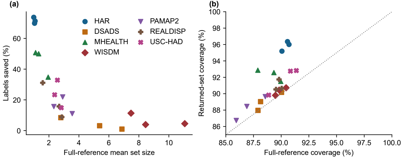
Fig. 7 Reference utility for LAC: (a) label savings versus reference set size; (b) returned-set versus reference coverage. Each point is a dataset-classifier mean; color and shape identify datasets. The diagonal denotes equal coverage
