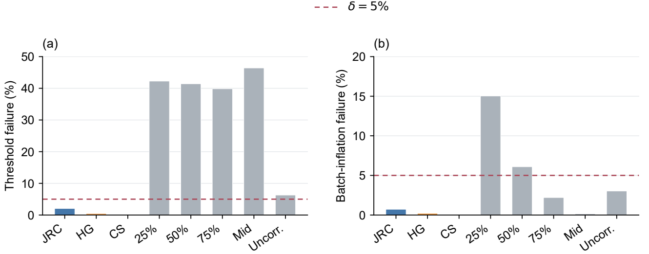
Fig. 3 USC-HAD LAC failures: (a) threshold failure; (b) monitoring-batch inflation above 0.5 labels. Dashed line: \delta = 5\% . Gray bars denote diagnostic rules; percentages denote query fractions. Mid: midpoint output; Uncorr.: uncorrected repeated looks
