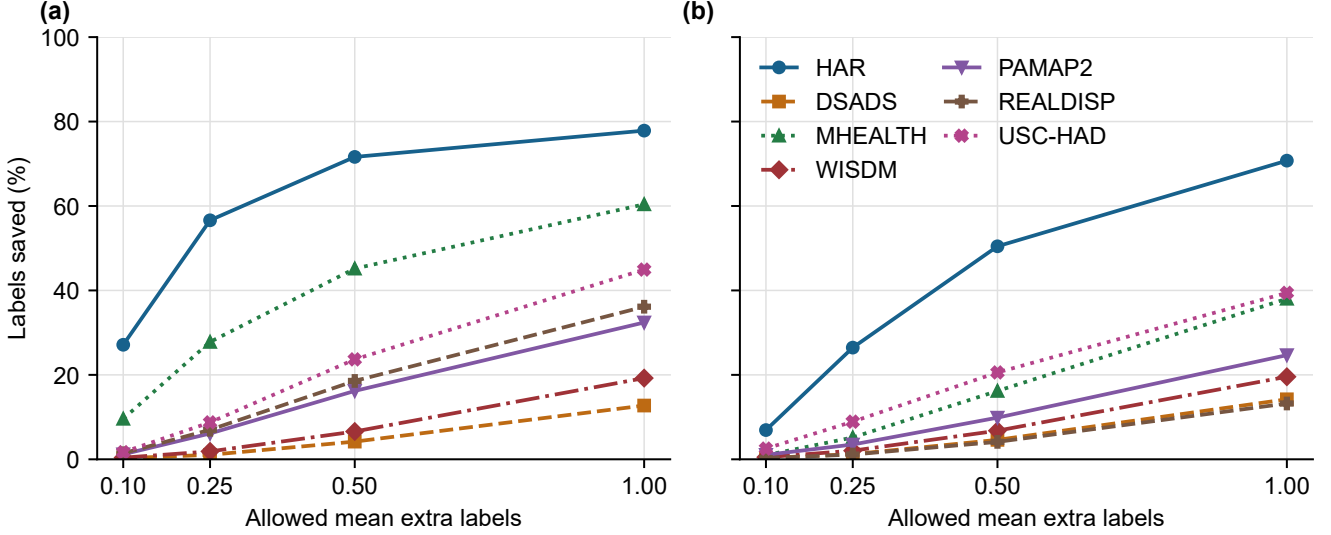
Fig. 5 Mean label savings of JRC versus the allowed extra set size: (a) LAC; (b) APS. Markers and line styles identify datasets
