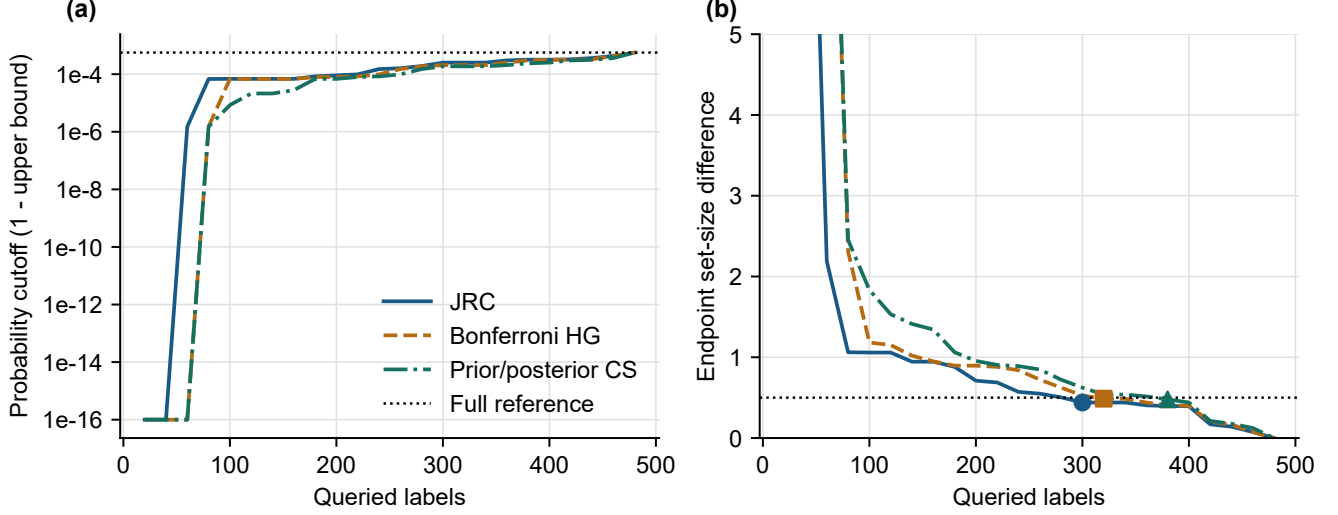
Fig. 6 USC-HAD MR query trace for LAC, N = 480 : (a) probability cutoff 1 - \bar{U}_t on a logarithmic scale; (b) endpoint set-size difference, with stopping locations marked. Zero cutoffs and infinite upper bounds are plotted at 10^{-16} . Horizontal line: \tau = 0.5
