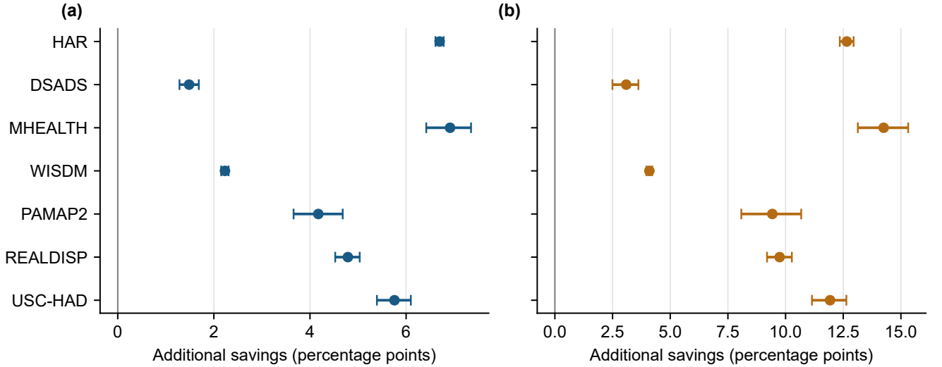
Fig. 4 Additional LAC label savings of JRC over (a) Bonferroni HG and (b) the uniform-prior CS. Points show paired participant means; bars show 95% bootstrap intervals
