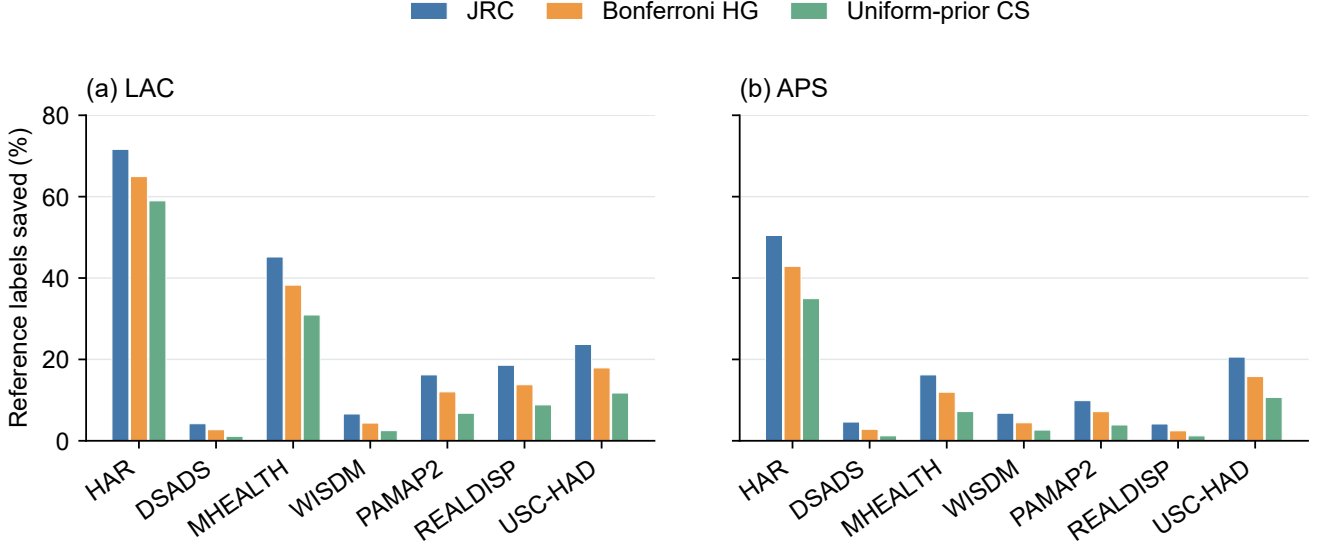
Fig. 2 Reference-label savings at \delta = 0.05 and \tau = 0.5 : (a) LAC; (b) APS. Bars show JRC, Bonferroni HG and the uniform-prior CS from left to right
