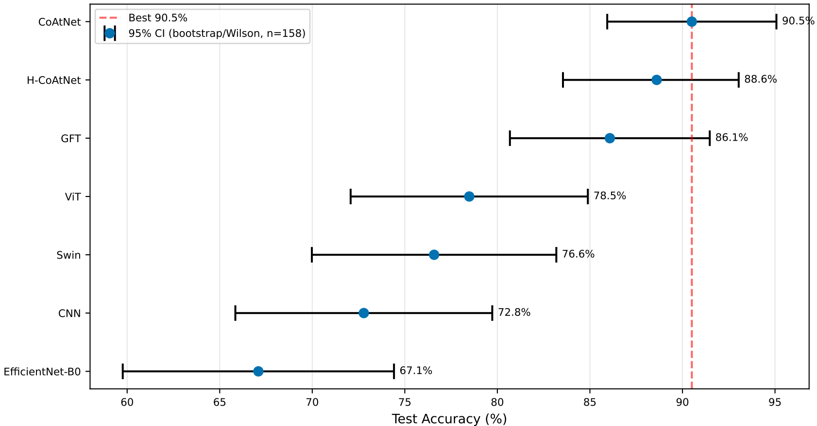
Forest Plot: Test Accuracy 95% CI per Model (n=158, stratified, seed 42)
