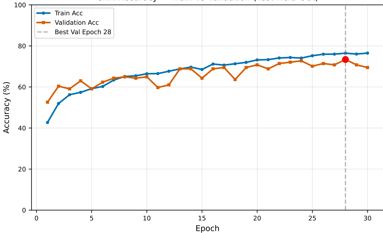
CNN Accuracy — Train vs Validation (Test Held-Out)
