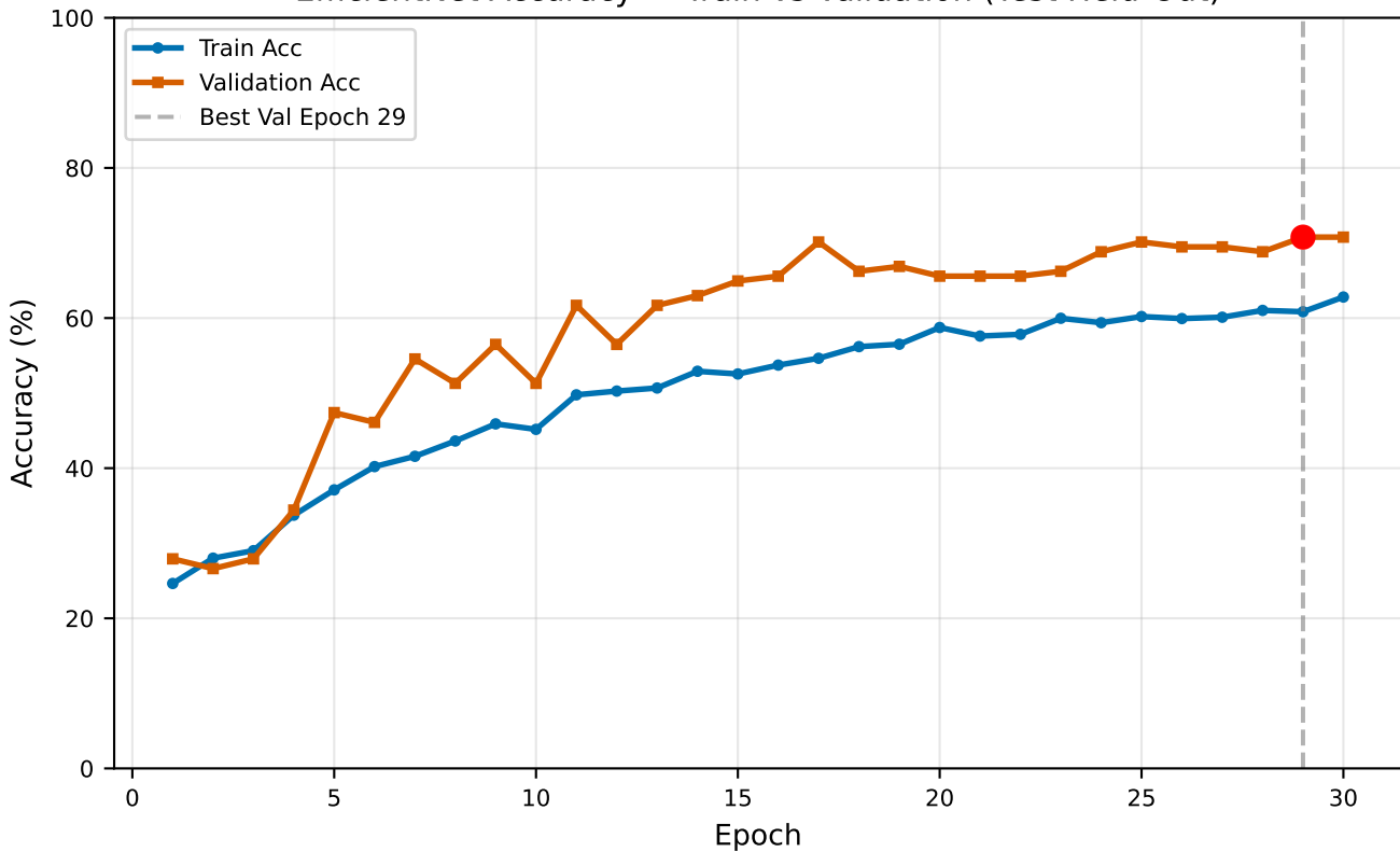
EfficientNet Accuracy — Train vs Validation (Test Held-Out)
