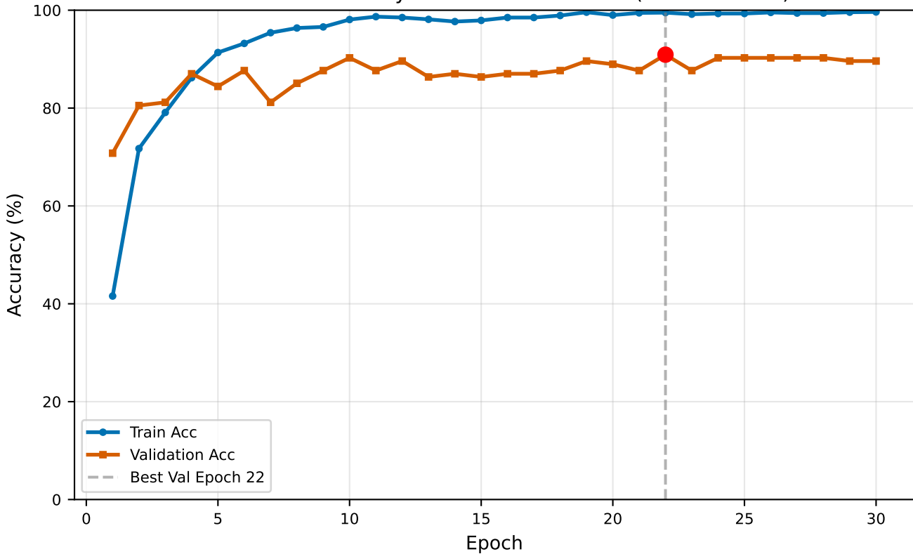
H-CoAtNet Accuracy — Train vs Validation (Test Held-Out)
