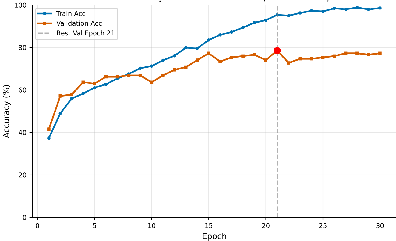
Swin Accuracy — Train vs Validation (Test Held-Out)
