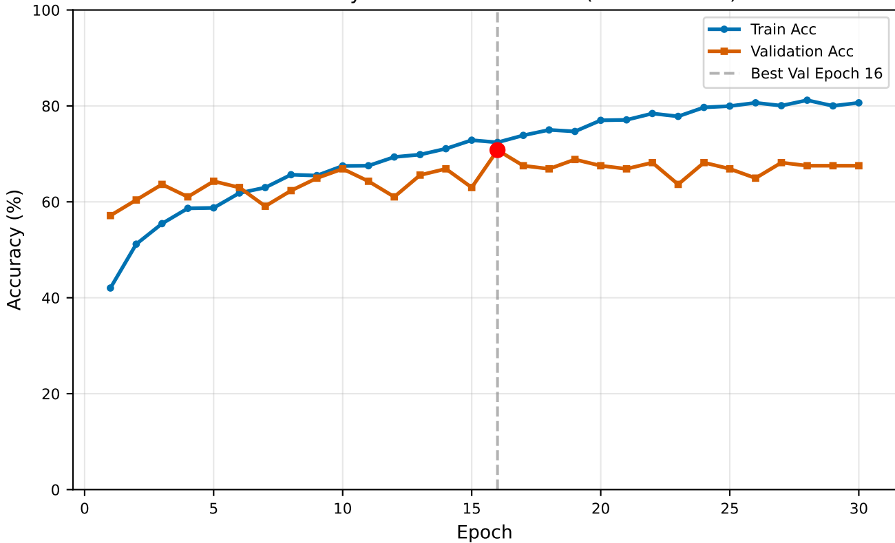
ViT Accuracy — Train vs Validation (Test Held-Out)
