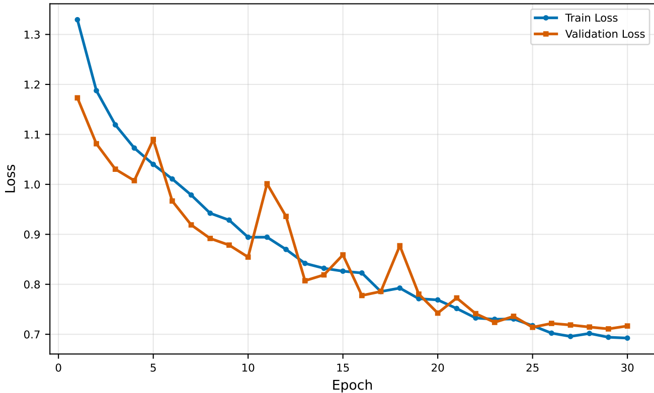
CNN Loss — Train vs Validation (Test Held-Out)
