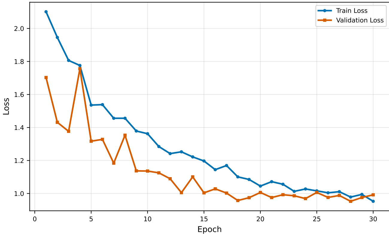
EfficientNet Loss — Train vs Validation (Test Held-Out)
