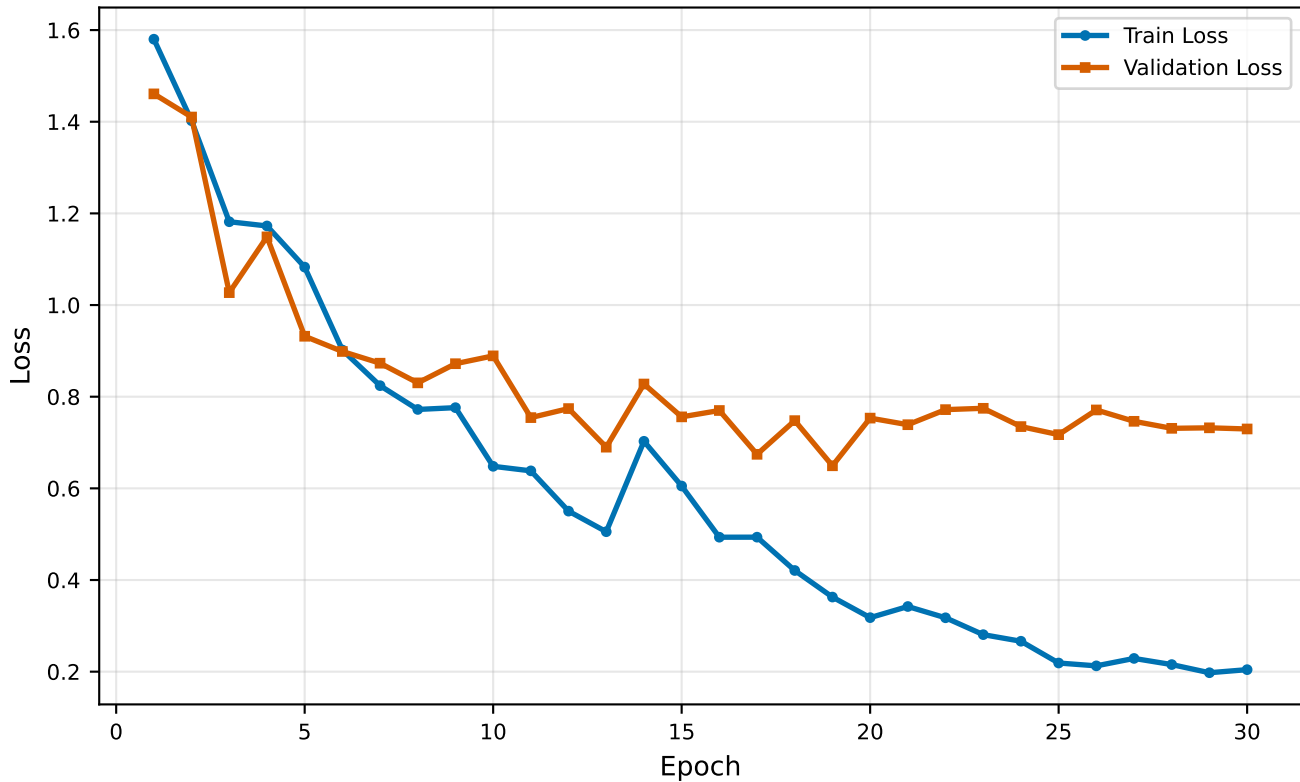
GFT Loss — Train vs Validation (Test Held-Out)
