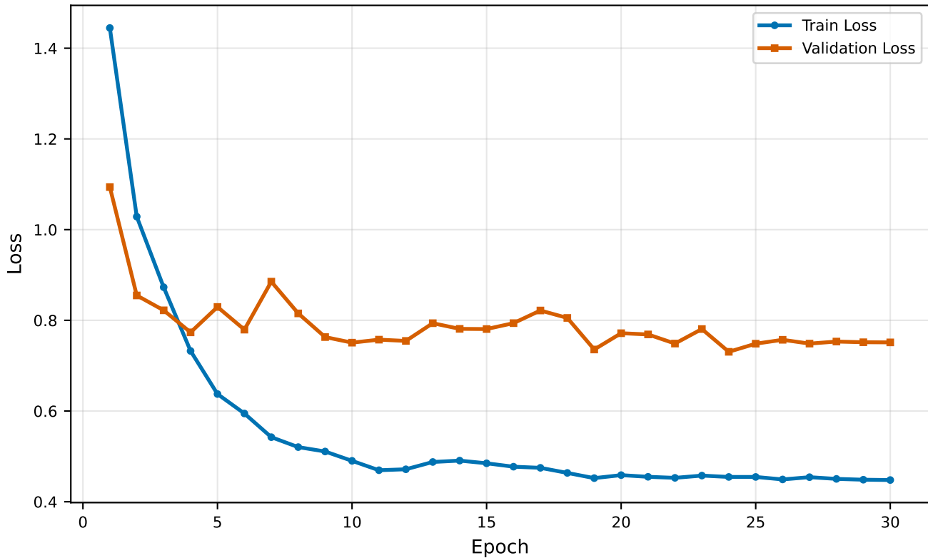
H-CoAtNet Loss — Train vs Validation (Test Held-Out)
