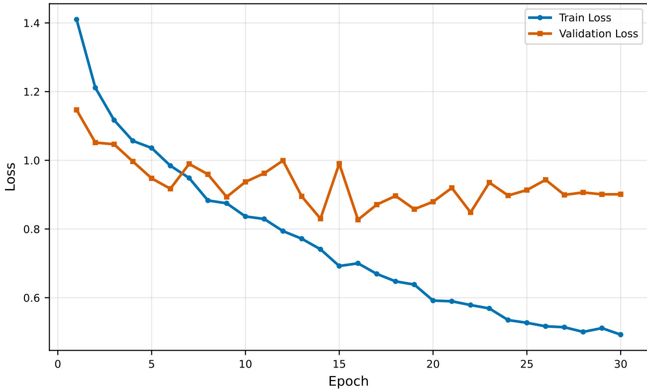
ViT Loss — Train vs Validation (Test Held-Out)
