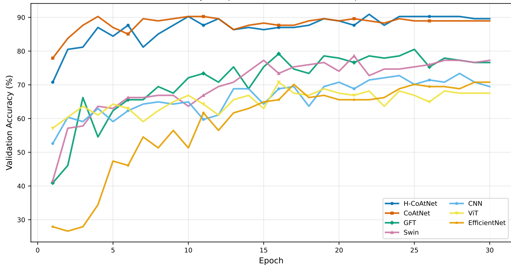
Validation Accuracy Comparison — All 7 Models (30 epochs, seed 42)
