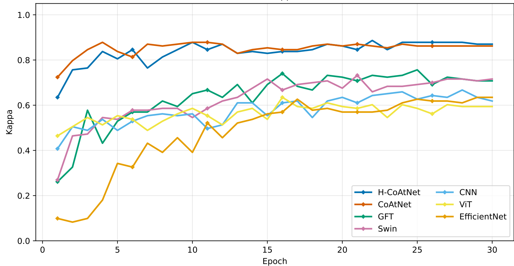
Validation Cohen's Kappa — All 7 Models
