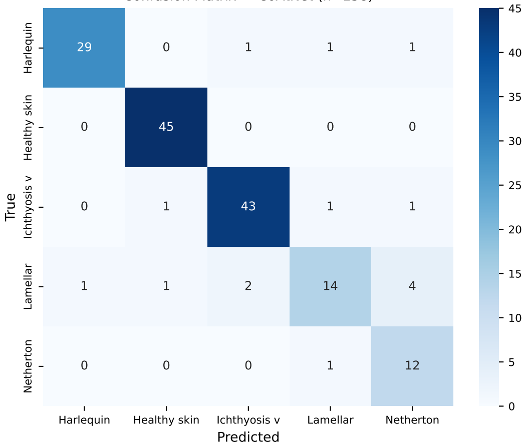
Confusion Matrix — CoAtNet (n=158)
