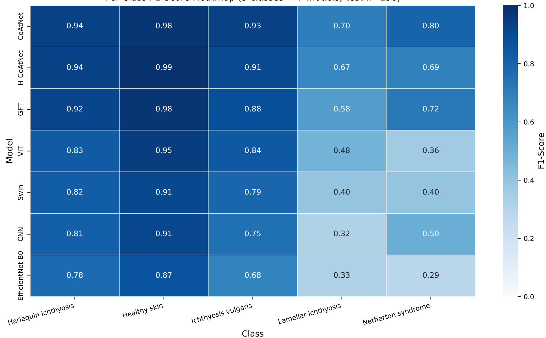
Per-Class F1-Score Heatmap (5 classes × 7 models, test n=158)
