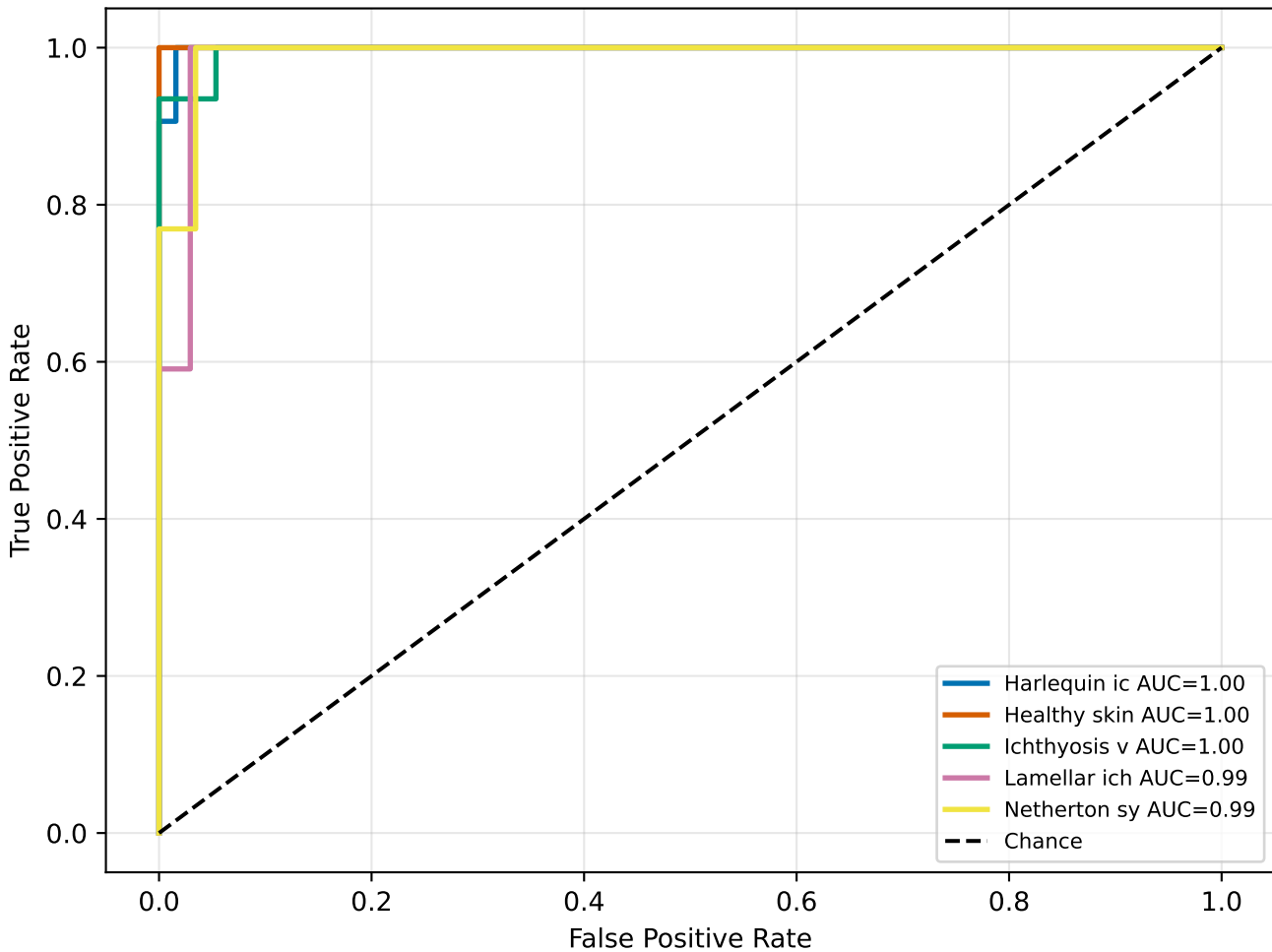
ROC (One-vs-Rest) — H-CoAtNet (Test n=158)
