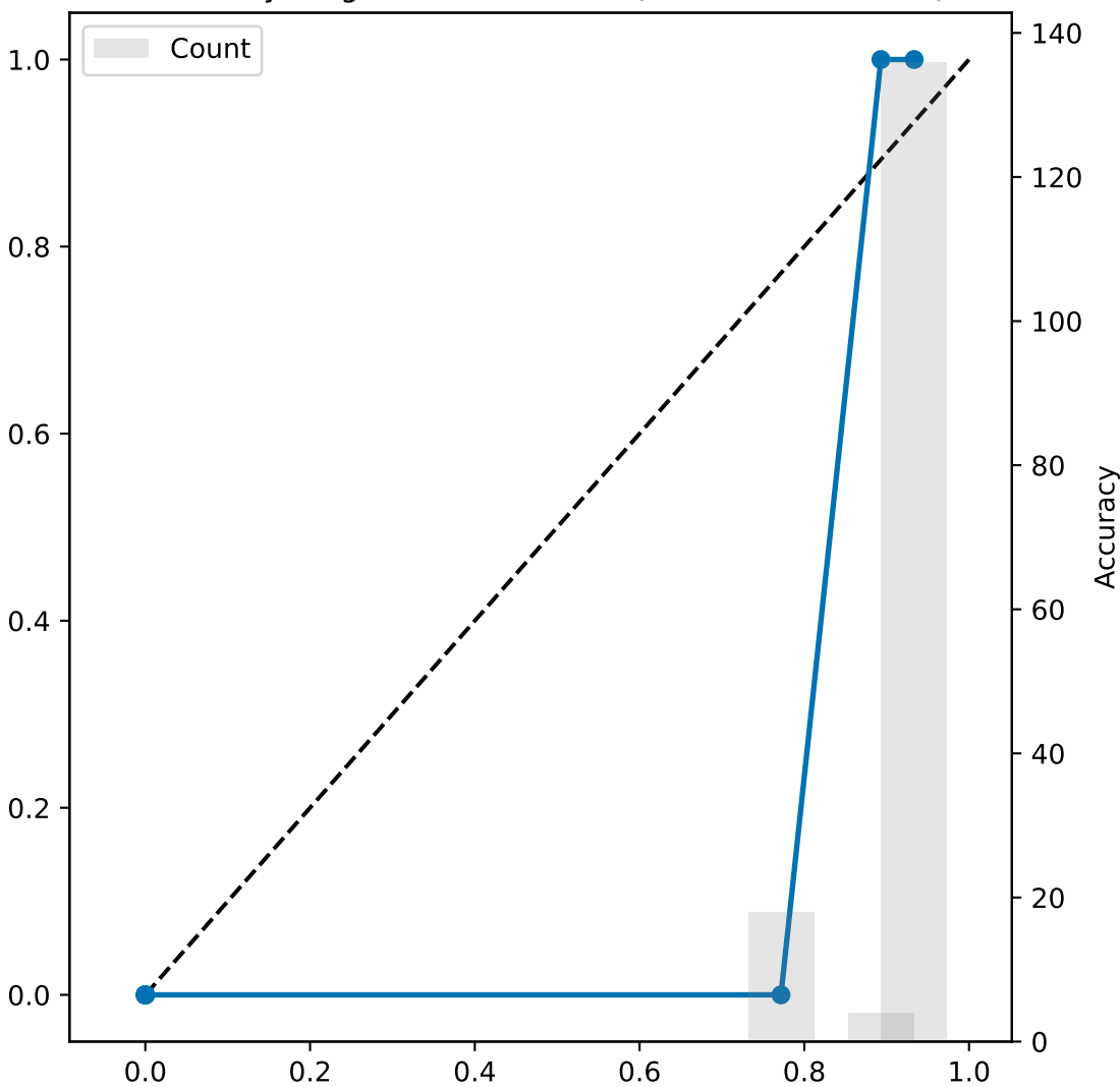
Reliability Diagram — H-CoAtNet (ECE=0.093, n=158)
