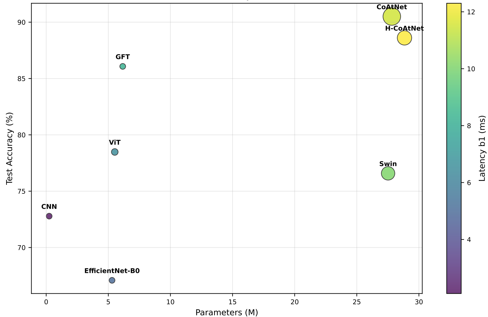
Efficiency vs Accuracy Trade-off Bubble size = MACs (G), Color = Latency b1 (ms) — Same HW/SW (T4)
