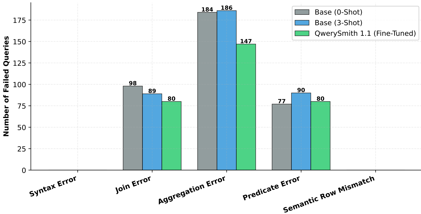
Figure 10: Comparative Failure Mode & Error Taxonomy Distribution
