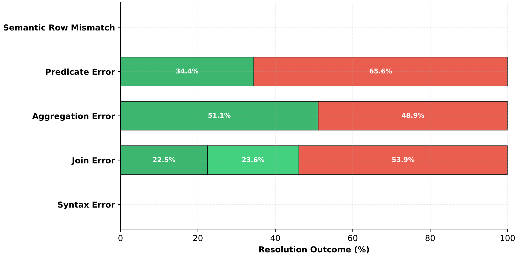
Figure 11: Error Recovery & Healing Matrix (Base Failures -> Fine-tuned Outcomes)
