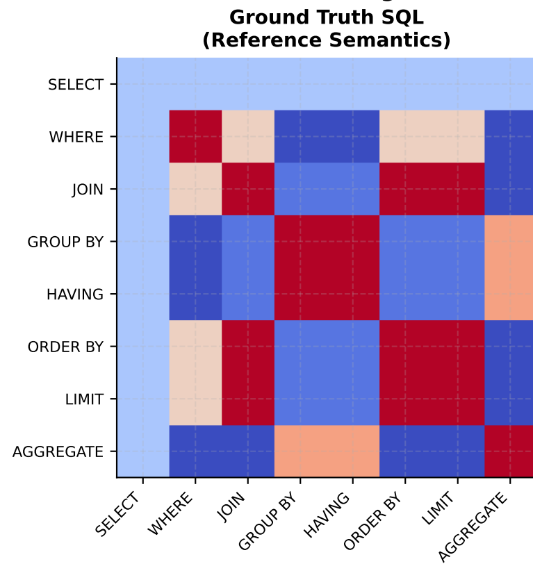
Figure 12: Cross-Clause Co-occurrence Correlation Matrix & Structural Alignment
