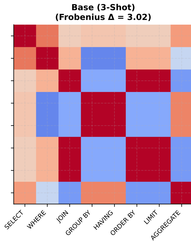
Figure 12: Cross-Clause Co-occurrence Correlation Matrix & Structural Alignment
