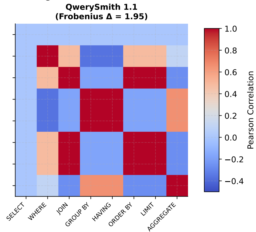
Figure 12: Cross-Clause Co-occurrence Correlation Matrix & Structural Alignment
